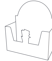
7268 3-3/4" Deep x 8-7/32 W x 4-31/32" H Built In Header Card Auto Bottom
