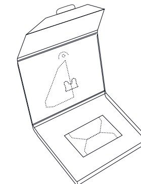
7408 8-13/16" W x 11-7/16" H 21/32" Capacity Box Panel Has Aperture to Hold Award Box Panel Has Optional EPS Foam Insert Easel Panel Has Clear Window Film, Holds Certificate Easel Panel Detaches from Box Panel For Display on table w. Easel Display on Wall w. Hang Tab Detached Easel is 11-7/16" W x 8-29/32" H Wrap Around Flap w. Tuck Tab
